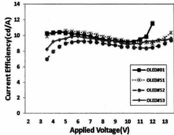
Fig. 4. Current efficiency-applied voltage characteristics of OLEDs with glass encapsulation on Alq 3 /LiF/Al buffer layers.
