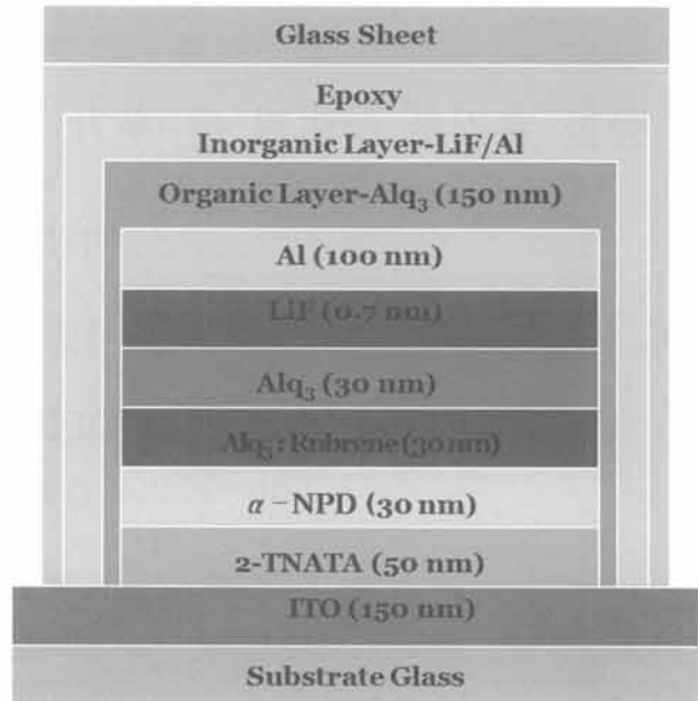
Fig. 1. Encapsulation structure of OLED with an organic-inorganic layer between OLED and glass sheet.
