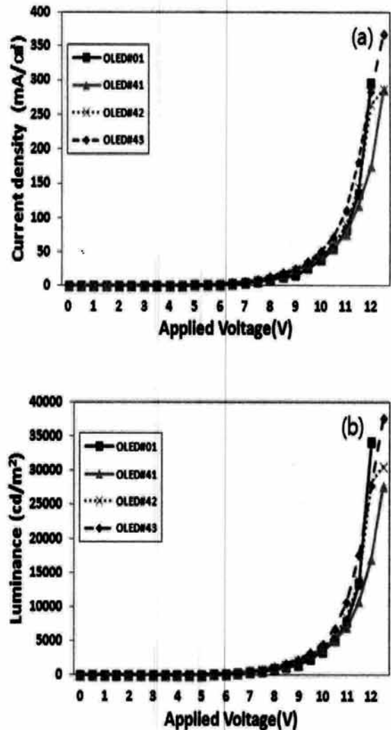
Fig. 2. Characteristics of OLEDs with Alq 3 /LiF/Al buffer layers. (a) current density–applied voltage, (b) luminance–applied voltage.
