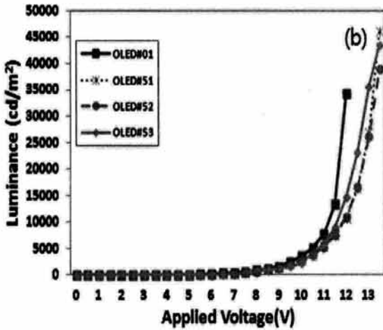
Fig. 3. Characteristics of OLEDs with glass sheet encapsulation on Alq 3 /LiF/Al buffer layers. (a) current density-applied voltage, (b) luminance-applied voltage.
