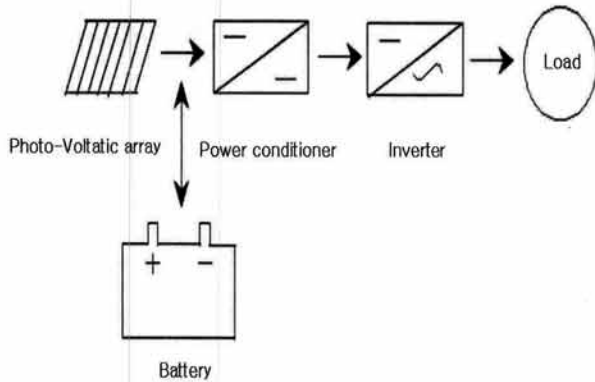
Fig. 1. Configuration of photovoltaic system.
