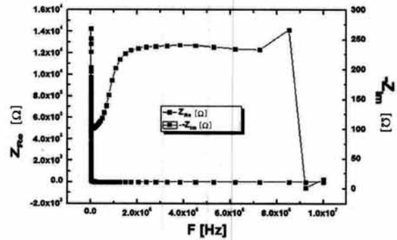
Fig. 7. Electrical characteristics of polycrystal silicon solar cell according to frequency variation.
