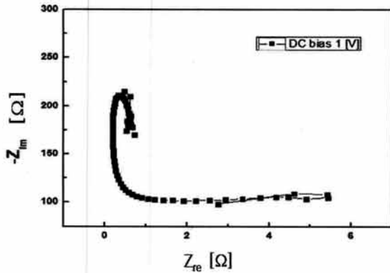
Fig. 5. Electrical characteristics of single crystal silicon solar cell according to frequency variation.
