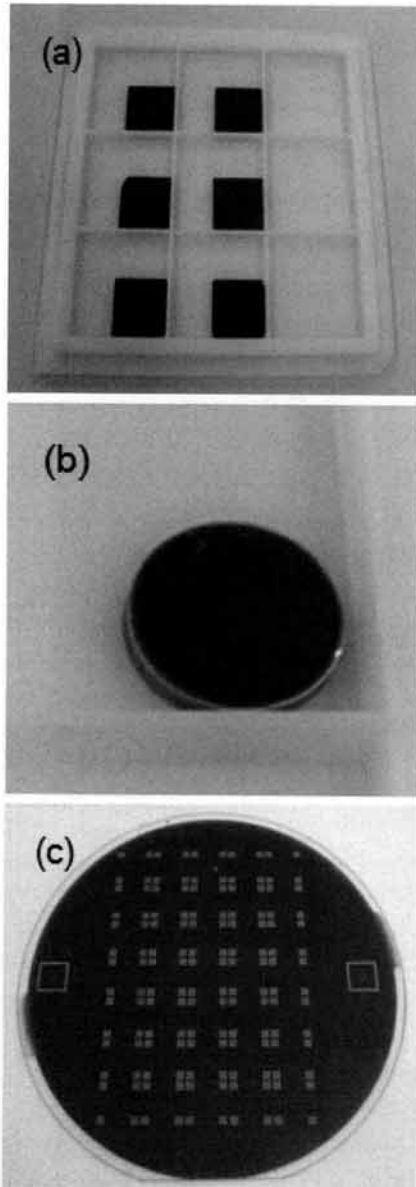
Fig. 1. Fabricated MDTF (a) deposition of MDTF on silicon wafer, (b) deposition of MDTF on germanium window, (c) deposition of MDTF on glass wafer for TCR measurement.
