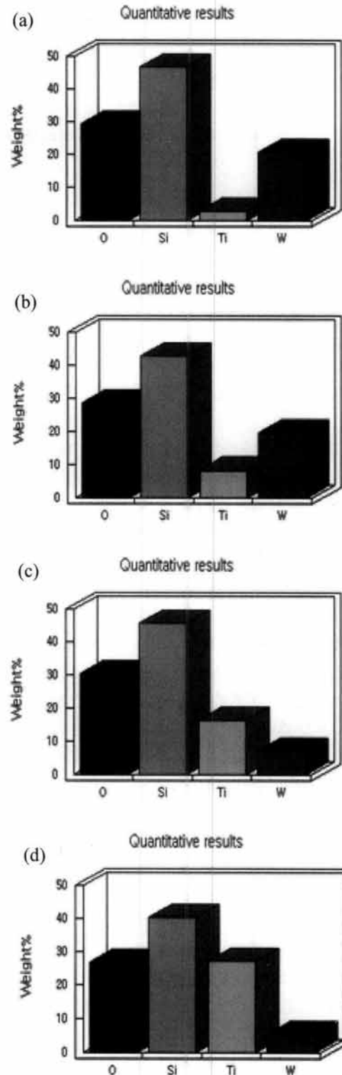
Fig. 4. EDAX analysis of element by mixing ratio of SiO_2-Ti , (a) (SiO_2)_{90}-(Ti)_{10} , (b) (SiO_2)_{80}-(Ti)_{20} , (c) (SiO_2)_{70}-(Ti)_{30} , (d) (SiO_2)_{60}-(Ti)_{40} .
