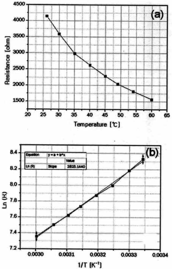
Fig. 5. (SiO 2 ) 70 -(Ti) 30 MDTF graph of the relationship between temperature and resistance (thickness 0.7 microns), (a) characteristics of resistance by MDTF temperature, (b) characteristics of resistance by MDTF temperature(1/T).
