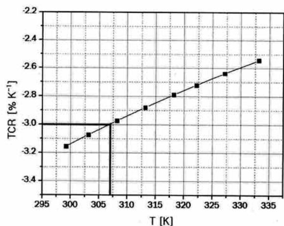
Fig. 6. TCR characteristics of (SiO 2 ) 70 -(Ti) 30 MDTF.
