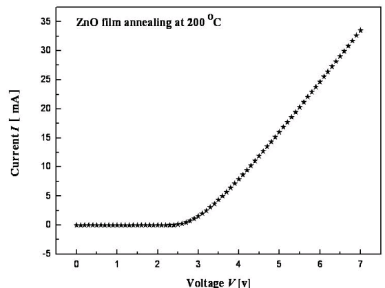
Fig. 1. The voltage-current of spin coated ZnO TCO on the PEN film.
