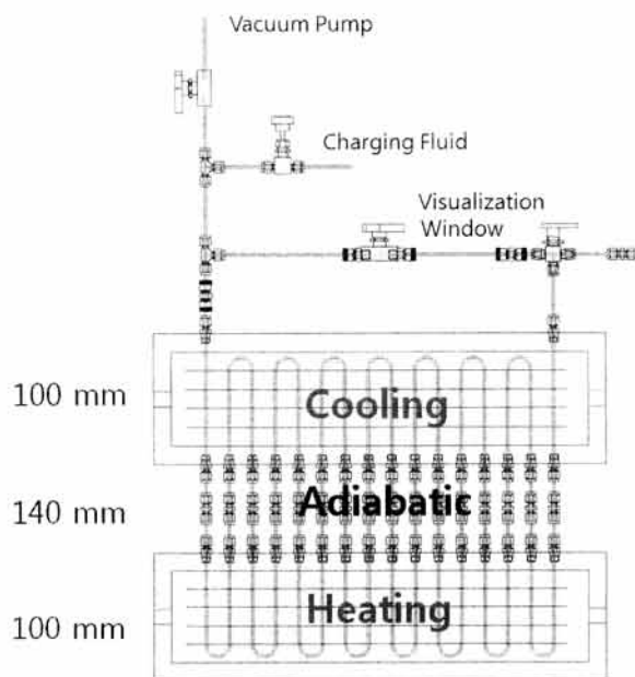
Fig. 3. Schematic of experimental apparatus.
