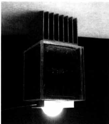
Fig. 2. Construction of 30 W explosion-proof LED light cooling system using pulsating heat pipe [11].
