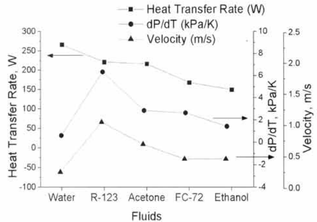
Fig. 7. Relations between heat transfer rate, ( dP/dT ), and velocity of working fluid.
