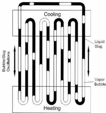
Fig. 1. Schematic of closed-loop type pulsating heat pipe.
