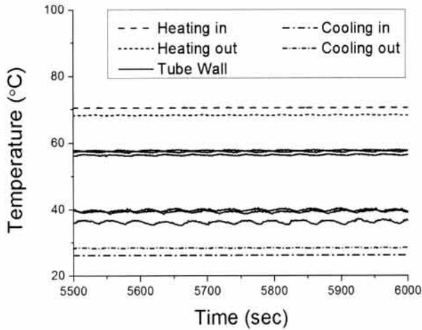
Fig. 5. Typical steady-state temperature signals (FC-72, 50%).
