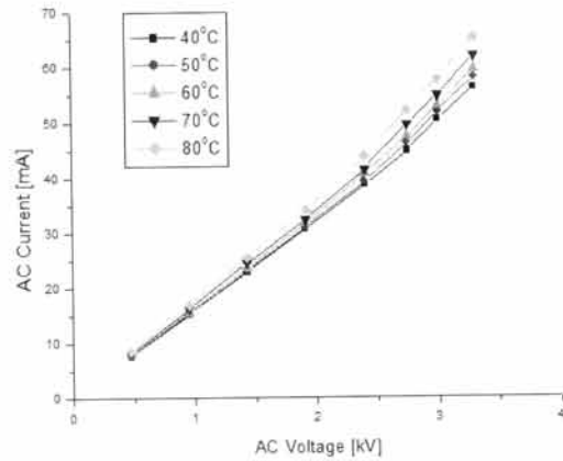
Fig. 6. AC current-voltage characteristics with various temperatures.
