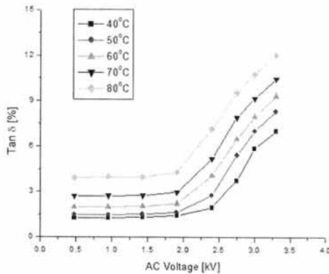
Fig. 7. \tan\delta -voltage characteristics with various temperatures.
