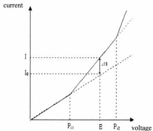
Fig. 2. Voltage-current curve.
