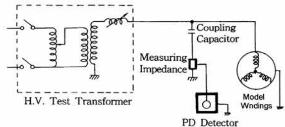
Fig. 5. Partial discharge measurement circuit.
