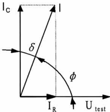
Fig. 4. Dissipation factor.
