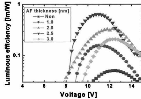
Fig. 6. Voltage-luminous efficiency depending on the thickness variation of Teflon-AF.
