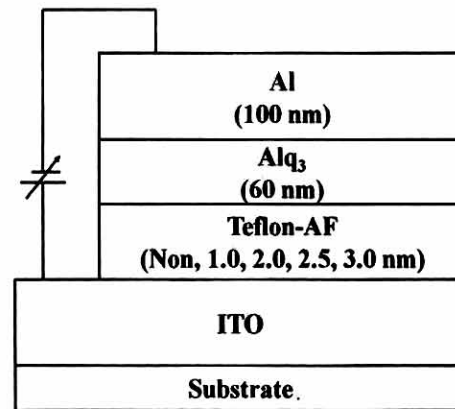
Fig. 2. Structure of the OLEDs.
