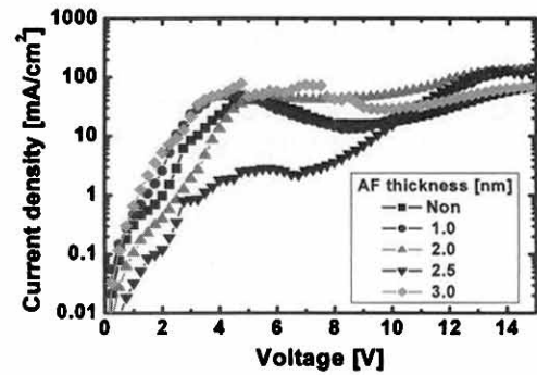
Fig. 4. Voltage-current density depending on the thickness variation of Teflon-AF.
