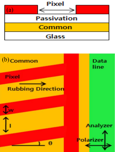
Fig. 2. (a) Cross-sectional and (b) top view of the conventional electrode structure of the FFS mode. The common electrode is located under the pixel electrode.
