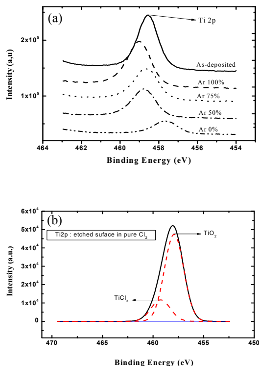
Fig. 4. (a) The spectrum of Ti2p with as variations of Ar/Cl 2 gas mixing ratio, (b) the deconvoluted Ti2p spectra at pure Cl 2
