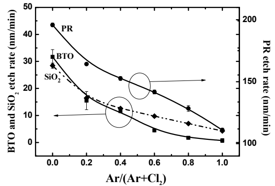
Fig. 1. Etch rate of BTO thin films and \text{SiO}_2 , PR as variations of \text{Ar}/\text{Cl}_2 gas mixing ratio.
