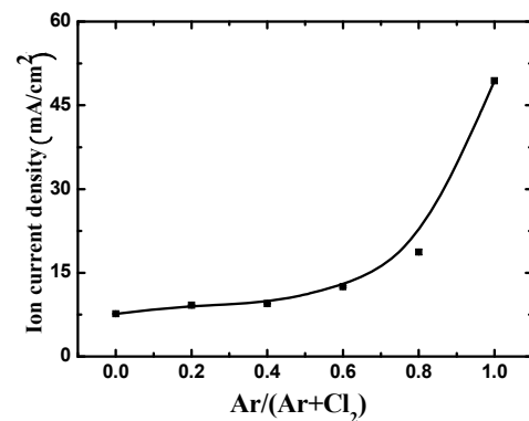
Fig. 2. Measured ion current density as variations of \text{Ar}/\text{Cl}_2 gas mixing ratio.
