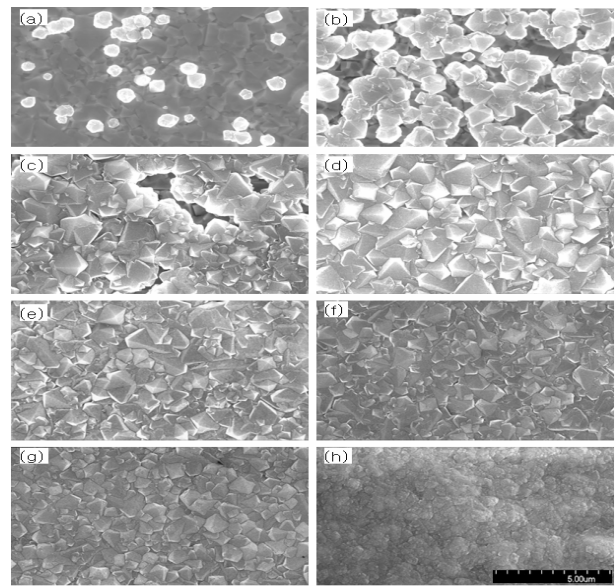
Fig. 1. The SEM micrographs of the films deposited with various \text{CH}_4 contents : (a) 10 sccm, (b) 20 sccm, (c) 30 sccm, (d) 40 sccm, (e) 50 sccm, (f) 75 sccm, (g) 100 sccm, and (h) 125 sccm.
