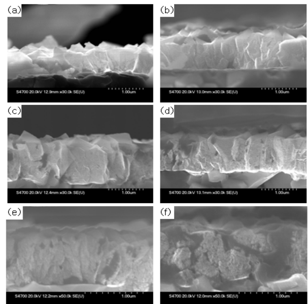
Fig. 2. The SEM micrographs showing cross-section morphologies of the films deposited with various \text{CH}_4 contents : (a) 30 sccm, (b) 40 sccm, (c) 50 sccm, (d) 75 sccm, (e) 100 sccm, (f) 125 sccm.
