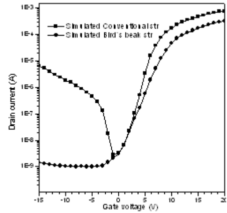
Fig. 4. The simulation result of Vg-Id transfer characteristics.
