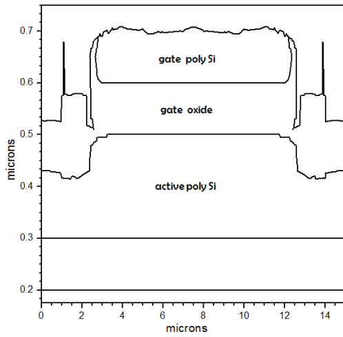
Fig. 2. The simulation result of TFT structure by Silvaco simulator.
