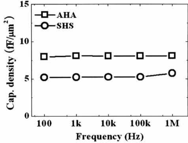
Fig. 3. Capacitance density of the sandwiched MIM capacitors as a function of frequency [11].
