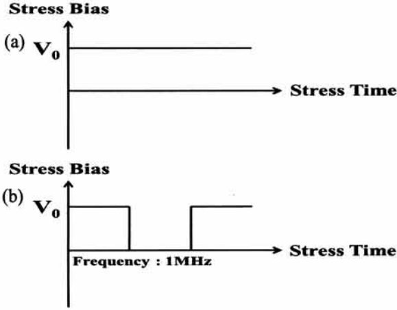
Fig. 2. Two kinds of voltage stress are applied to analyze the dependence of capacitance variation on stress type. (a) DC voltage stress and (b) AC voltage stress.
