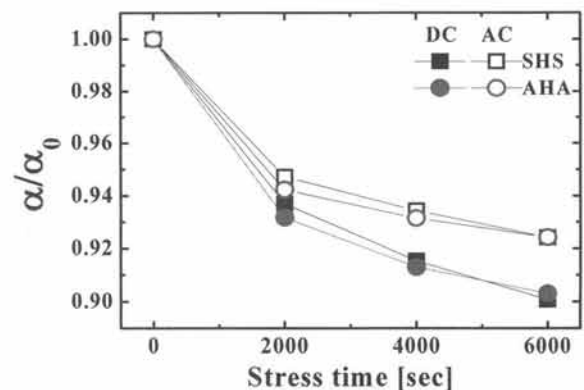
Fig. 7. Variation of VCC for two sandwiched MIM capacitors as a function of stress time under DC and AC stresses (solid : DC stress, open : AC stress).
