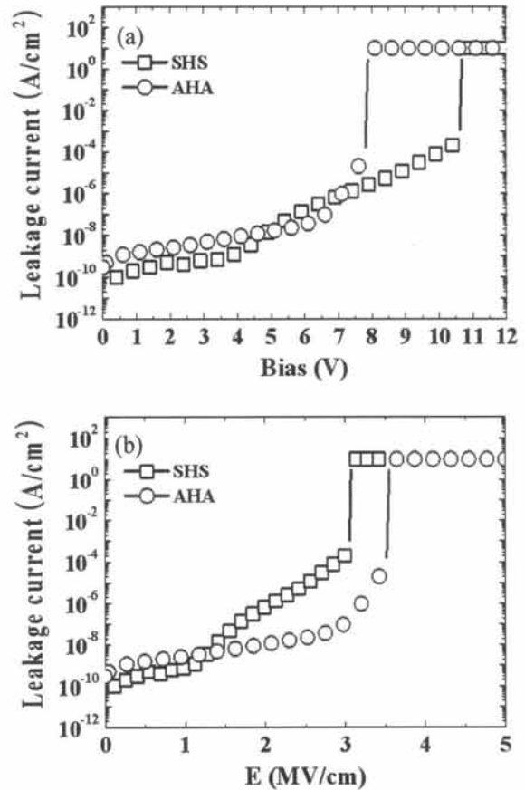
Fig. 4. (a) Leakage current versus applied bias, and (b) leakage current versus electric field for two sandwiched MIM capacitors. Electric field in (b) was obtained by dividing the applied bias in (a) by the effective thickness of dielectrics expressed as (1) and (2).
