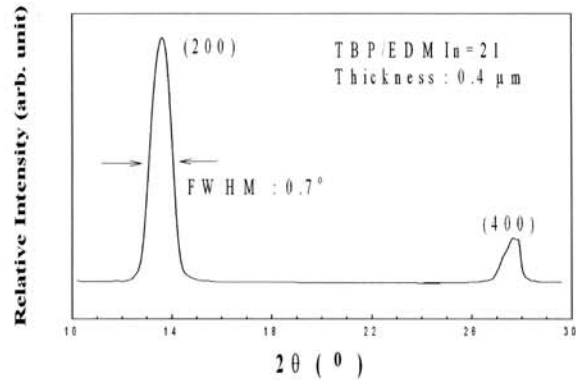
Fig. 3. An XRD pattern of an InP epitaxial layer grown at 550°C with a TBP/EDMIn molar ratio of 21 under atmospheric pressure.
