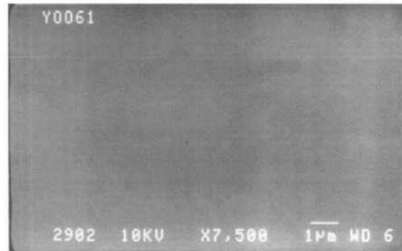
Fig. 4. An SEM photograph of an InP epitaxial layer whose XRD pattern is shown in Fig. 3.
