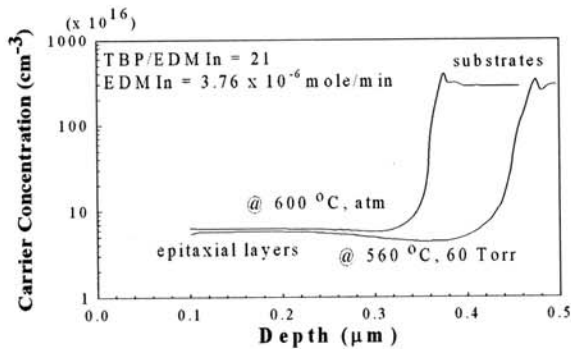
Fig. 6. Carrier concentration profiles of InP epitaxial layers.
