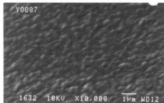
Fig. 5. An SEM photograph of an InP epitaxial layer grown at 480°C with a TBP/EDMIn molar ratio of 40 under atmospheric pressure.
