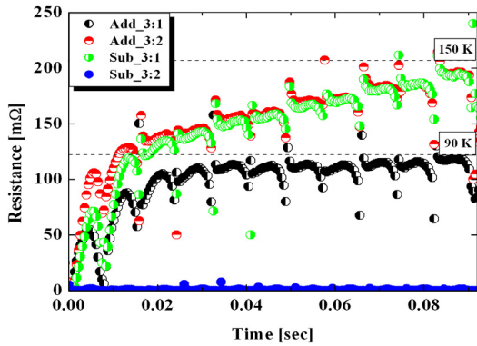
Fig. 5. Resistance characteristics of the YBCO@Sus CC according to connection type of the coil.
