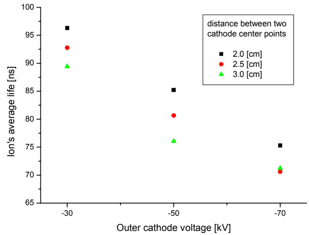
Fig. 6. Ion's average lives according to a variation of voltages applied to the outer grid cathode and distances between two cathodes.
