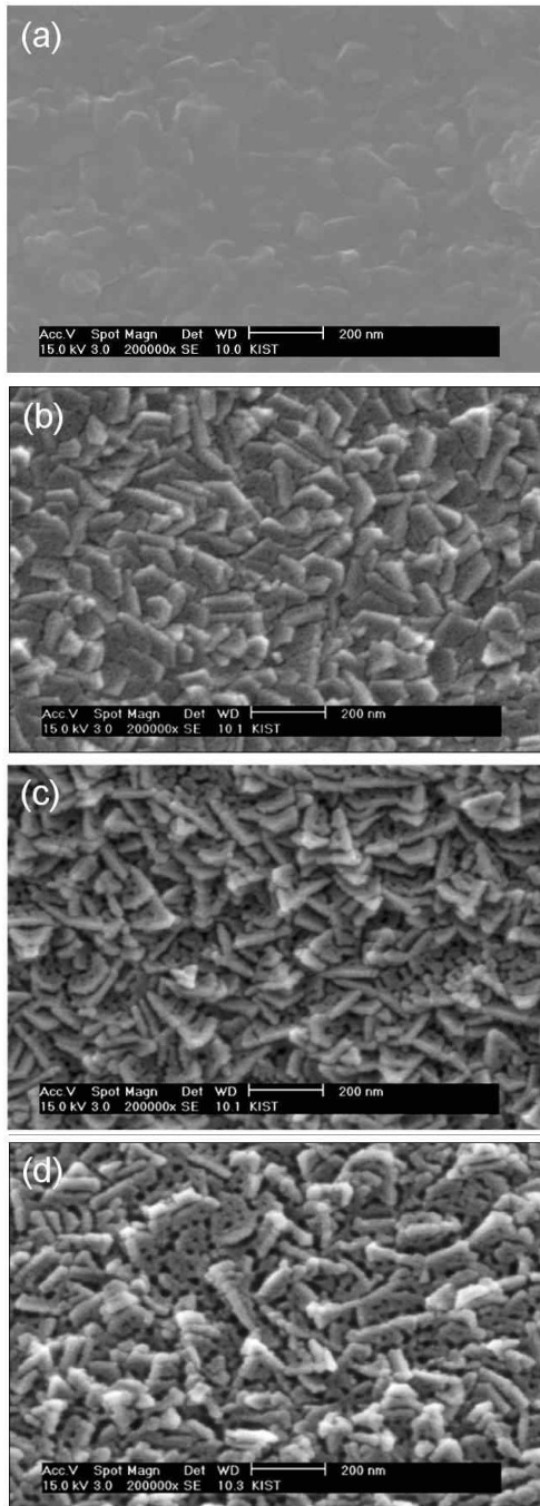
Fig. 2. Plain-view SEM images of Ti thin films (a) before and (b) after anodization for (b) 15 min, (c) 1 h, and (d) 3 h.
