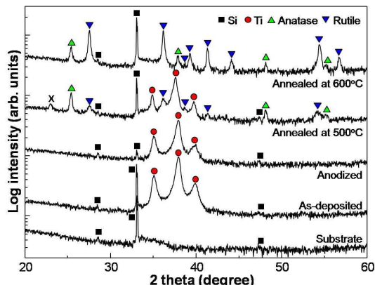
Fig. 5. Out-of-plane \theta - 2\theta XRD patterns of Si substrate, Ti thin film, anodized Ti film, anodized films after annealed at 500°C and 600°C.
