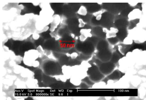
Fig. 4. Plain-view SEM image of the anodized Ti film for 3 h after the removal of surface oxide layer by Ar ion beam etching for 2 min.
