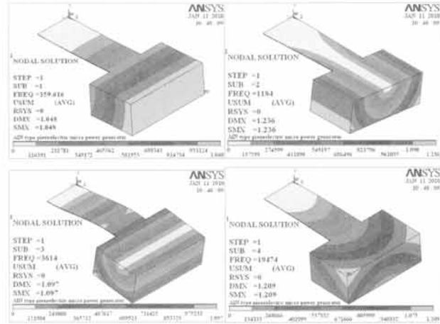
Fig. 5. Strain distributions of AlN micro energy harvesters with bending modes.
