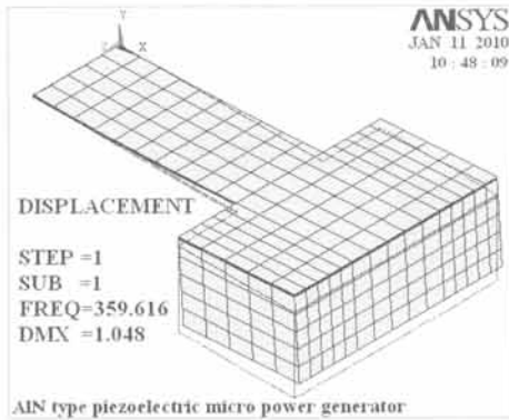
Fig. 4. Optimal modal of designed AlN micro energy harvester.
