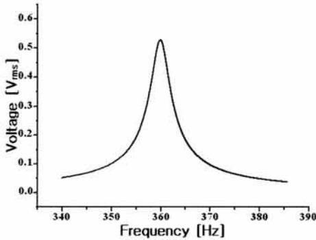
Fig. 7. Output voltage variations of AlN micro energy harvester with frequency.
