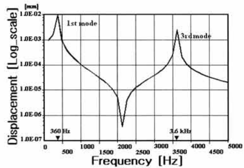
Fig. 6. Displacements of AlN micro energy harvesters with frequency range.
