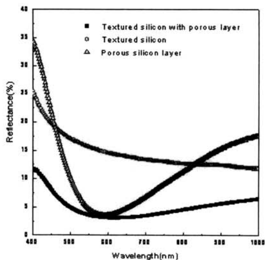
Fig. 4. The reflectance of textured monocrystalline silicon with and without the porous Si layer.
