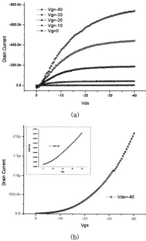
그림 5. 제작된 P3HT/POSS OTFT의 (a) 출력특성 (b) 전달특성. (채널길이 : 15 μm, 넓이 : 1 mm, V_{th} = -6.54 \text{ V} , \mu_{fet} = 1.19 \times 10^{-3} \text{ cm}^2/\text{V}\cdot\text{s} , I_{on/off} ratio : 2.51 \times 10^2 ) Fig. 5. (a) Output characteristic and (b) transfer characteristic of the P3HT/POSS OTFT. (Channel Length : 15 μm, Width : 1 mm, V_{th} = -6.54 \text{ V} , \mu_{fet} = 1.19 \times 10^{-3} \text{ cm}^2/\text{V}\cdot\text{s} , I_{on/off} ratio : 2.51 \times 10^2 )
