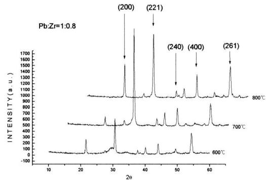
그림 2. Pb:Zr=1:0.8에서 온도에 따른 XRD. Fig. 2. XRD with different annealing temperature of PbZrO 3 films that mole ratio of Pb:Zr is 1:0.8.
