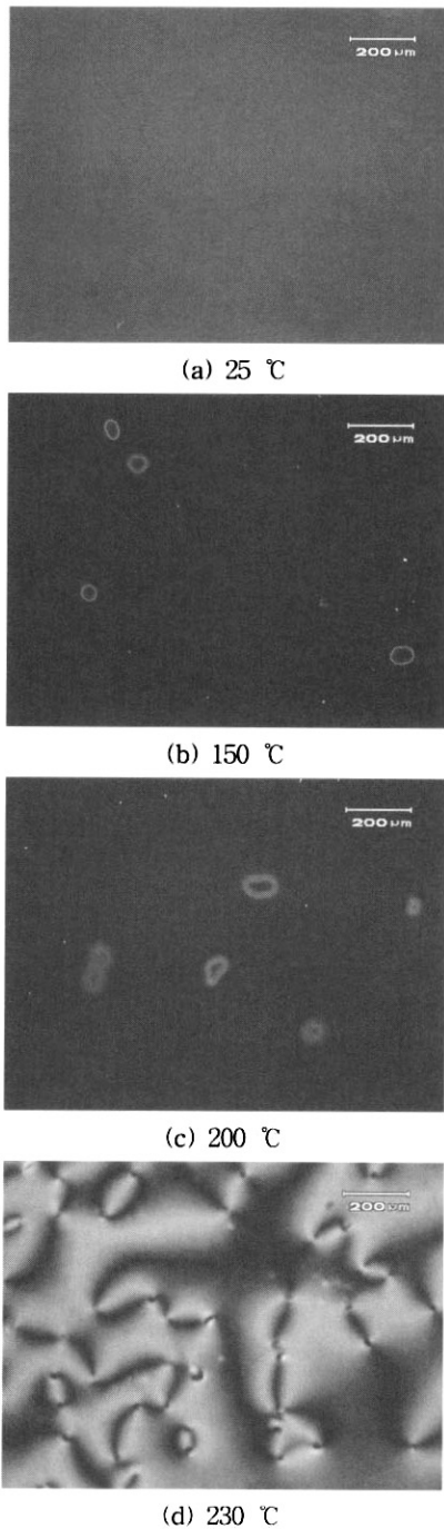
Fig. 5. Microphotographs of aligned LC on the organic overcoat thin film surface with ion beam irradiation of 60^\circ for 2 min at various annealing temperatures (in crossed Nicols).
