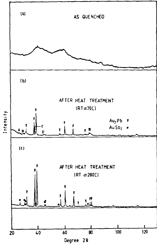
Fig.3 X-ray diffraction pattern of amorphous Pb-Sb-Au alloys. (a) as quenched (b) after heat treatment of 70 °C (c) after heat treatment of 280 °C. (RT: Room Temp.)
