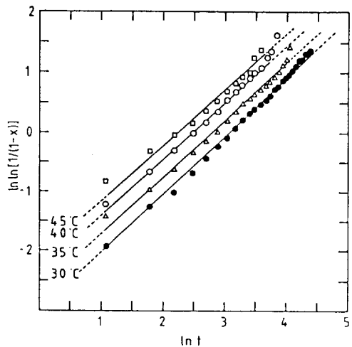
Fig.5 Plot of \ln\{x/(1-x)\} vs \ln t for amorphous (Pb_{0.75}Sb_{0.25})_{45}Au_{55} alloy.
