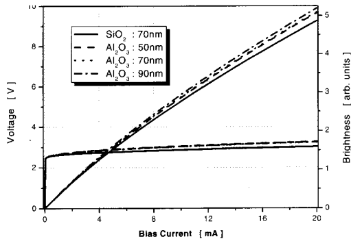
Fig. 3. L-I-V curves of packaged LED lamps with passivation layers
