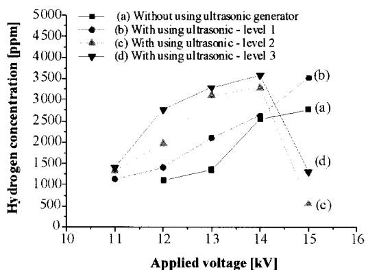
Fig. 5. The comparison of the hydrogen concentration in cases of using ultrasonic wave generator under N_2 and 10 mL water quantities.
