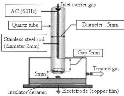
Fig. 1. Schematic diagram of the plasma reactor.
