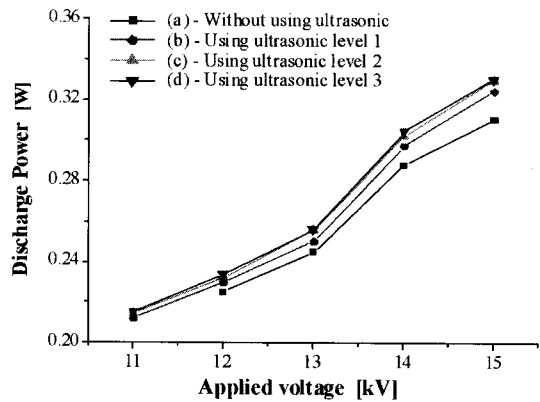
Fig. 3. The relationship between the power consumption and the applied voltage.
