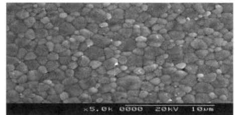
(b) 2 mol%
