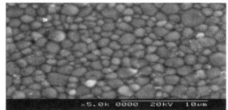
(c) 3 mol%
