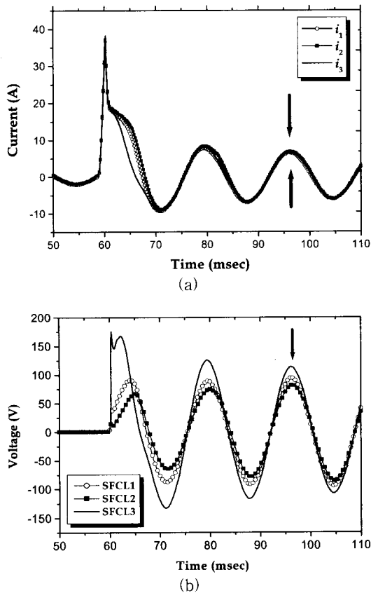
그림 4. 하이브리드형 SFCL의 전기적 특성(전원 전압 : 220 V rms ). Fig. 4. Electrical properties of SFCL units in a hybrid type SFCL (applied voltage: 220 V rms ). (a) Current curves of three SFCLs. (b) Voltage curves of three SFCLs.
