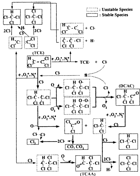
(a) Chemical reaction in the plasma region
