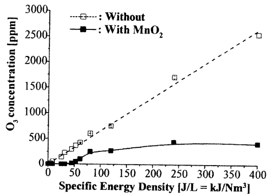
(b) The change of ozone concentration
