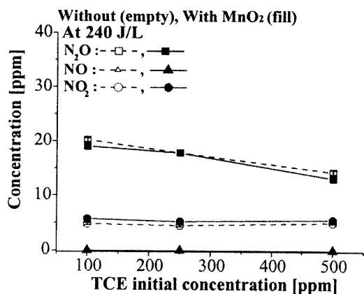
(c) The change of N_xO_y ( NO , NO_2 , N_2O )
