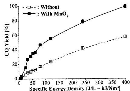
(b) The change of CO x yield (%)
