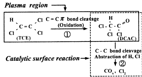
(b) The expected chemical reactions
