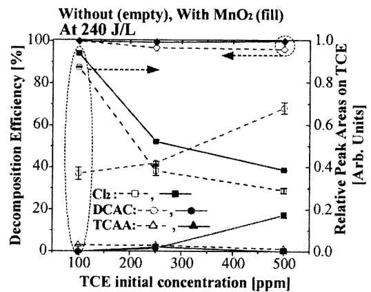
(b) The change of chlorine contained-byproducts
