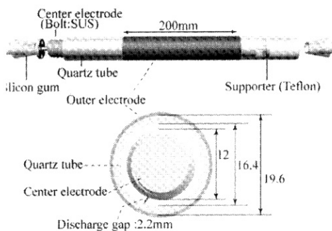
Fig. 2. Schematics of experimental setup and the barrier discharge reactor.
