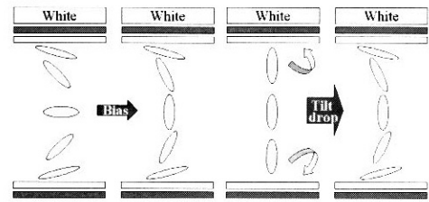
(a) Principal of the OCB cell (b) Structure of the novel HTOCB cell
