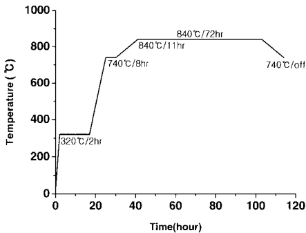
Fig. 1. Process abridged general view.
