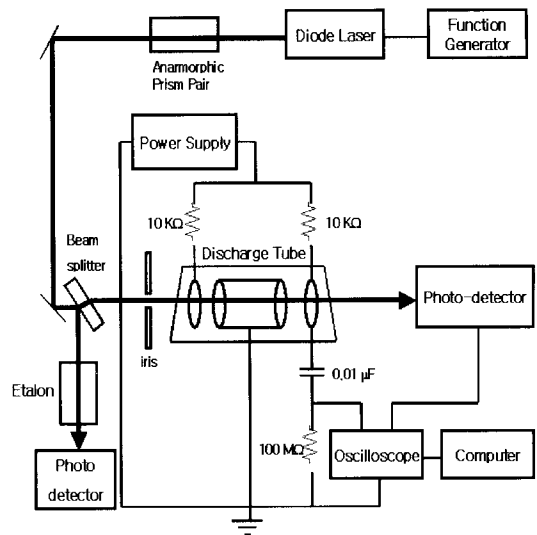
Fig. 1. Experimental setup.
