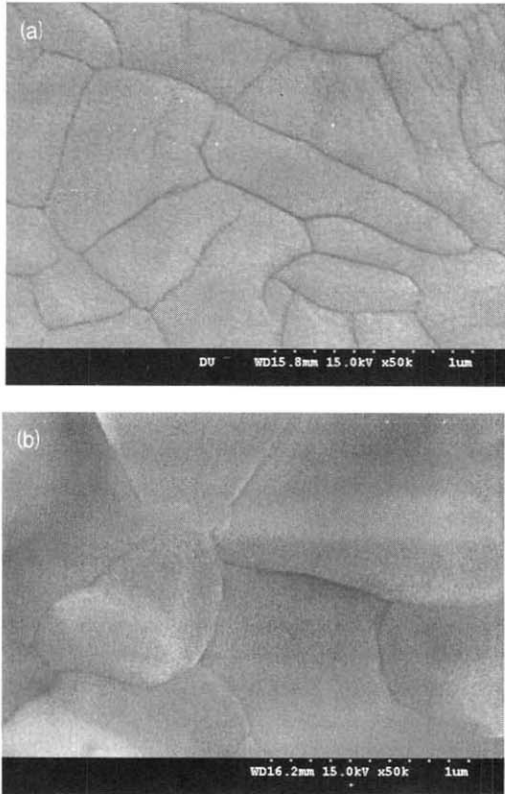
그림 2. \text{La}_2\text{Mo}_{2-x}\text{Nb}_x\text{O}_9 의 주사전자현미경 사진; (a) \text{La}_2\text{Mo}_2\text{O}_9 and (b) \text{La}_2\text{Mo}_{1.9}\text{Nb}_{0.1}\text{O}_{9.6} . Fig. 2. Scanning electron micrographs of \text{La}_2\text{Mo}_{2-x}\text{Nb}_x\text{O}_9 ; (a) \text{La}_2\text{Mo}_2\text{O}_9 and (b) \text{La}_2\text{Mo}_{1.9}\text{Nb}_{0.1}\text{O}_{9.6} .
