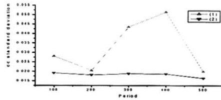
(b) Cross correlation standard deviation according to period
