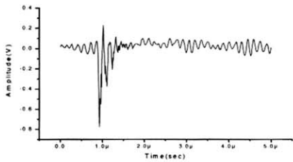
(a) Waveform & FFT at Needle-Plane Electrodes
