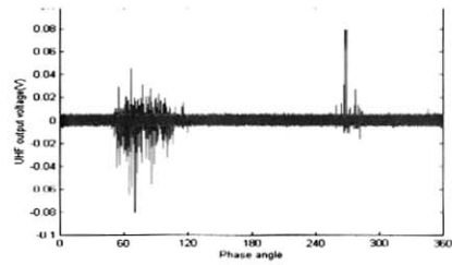
(b) PD pulses during 100 period (Needle-Needle)
