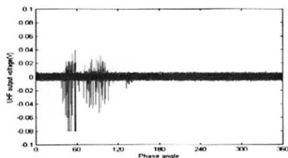
(a) PD pulses during 100 period (Needle-Plane)
