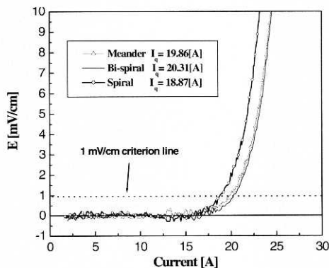
Fig. 3. E-I curves of individual SFCL elements with pattern shapes.
