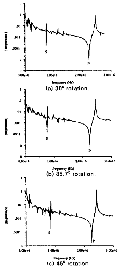
Fig. 5. Variation of impedance analyzed with finite element method.
