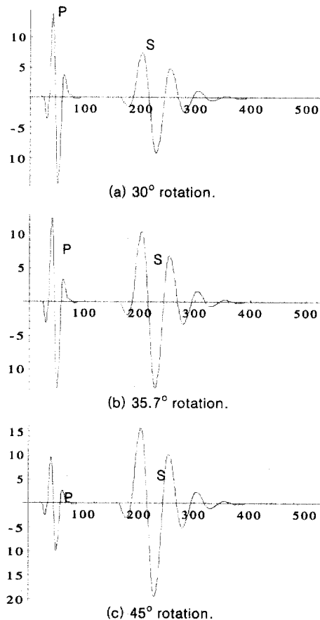
Fig. 8. Pulse-echoed waves for each rotation angle.
