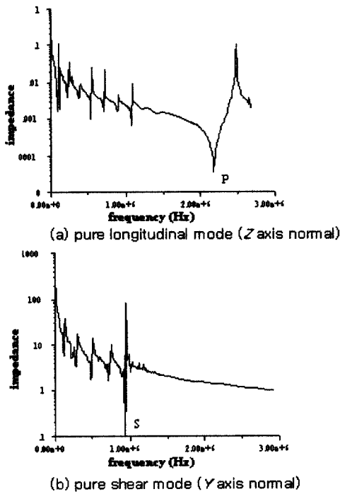
Fig. 4. Impedance variation of the PZT element with different crystal cut directions.
