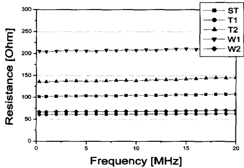
(b) 저항
