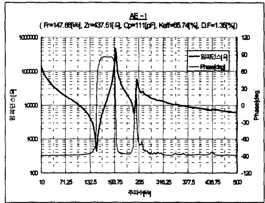
(a) AE-1(8.1 mm \phi \times 8.1 mm) 센서
