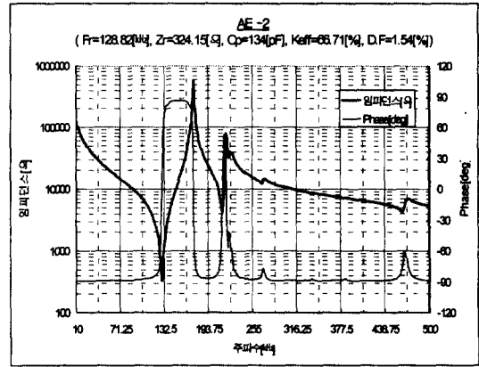
(b) AE-2(9.5 mm \phi \times 9.5 mm) 센서
