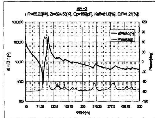
(c) AE-3(14.3 mm \phi \times 14.3 mm) 센서
