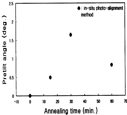
(b) filling in isotropic phase.
