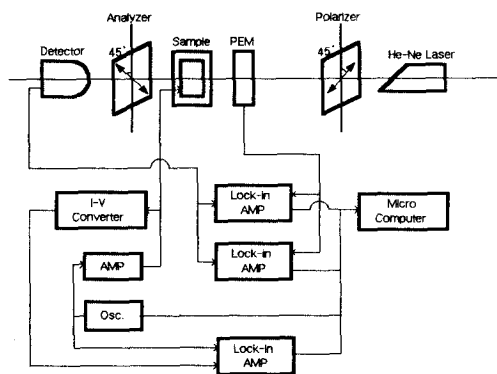
Fig. 2. Measuring system of anchoring strength.
