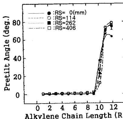
Fig. 3. Generation of pretilt angle of 5CB on rubbed PTP surfaces as a function of alkyl chain lengths.
