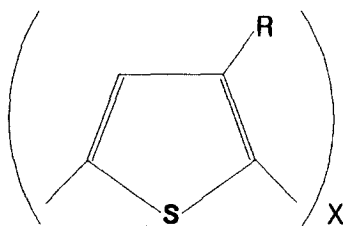
Fig. 1. Molecular structure of thiophene.
