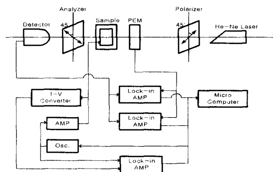
Fig. 2. Measuring system of polar anchoring strength.
