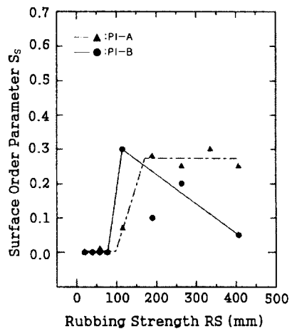
Fig. 6. Surface order parameter of 5CB on two kinds of the rubbed PI surfaces as a function of RS.
