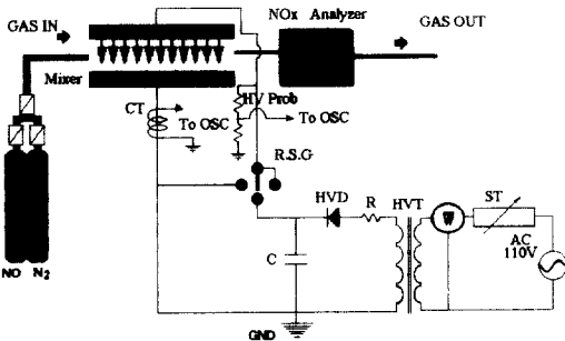
FM : flow meter HVD : high voltage diode ST : sliduces C : capacitor[33.6 μF] OSC : oscilloscope(powerpro 610) W : powermeter R.S.G : rotating spark gap switch HVT:high voltage transformer R:stability resistance[50K Ω]
