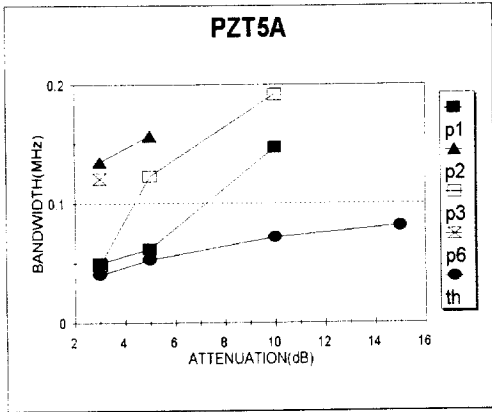
(c) PZT5A
