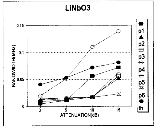
(a) LiNbO 3
