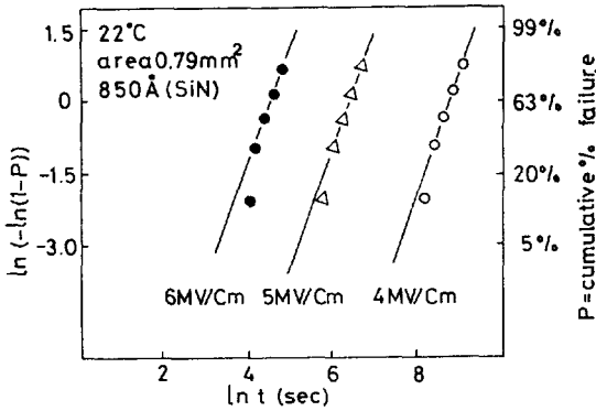
Fig. 7. Wearout curve of MNS capacitor as a parameter of stress field.
