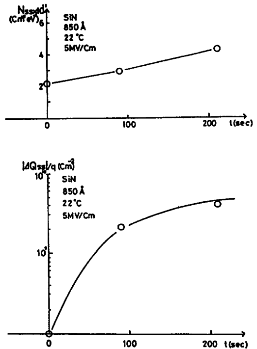
Fig. 14. The change of characteristics of SiN film as a function of stress time.
