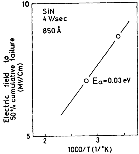
Fig. 6. Activation energy of breakdown strength.
