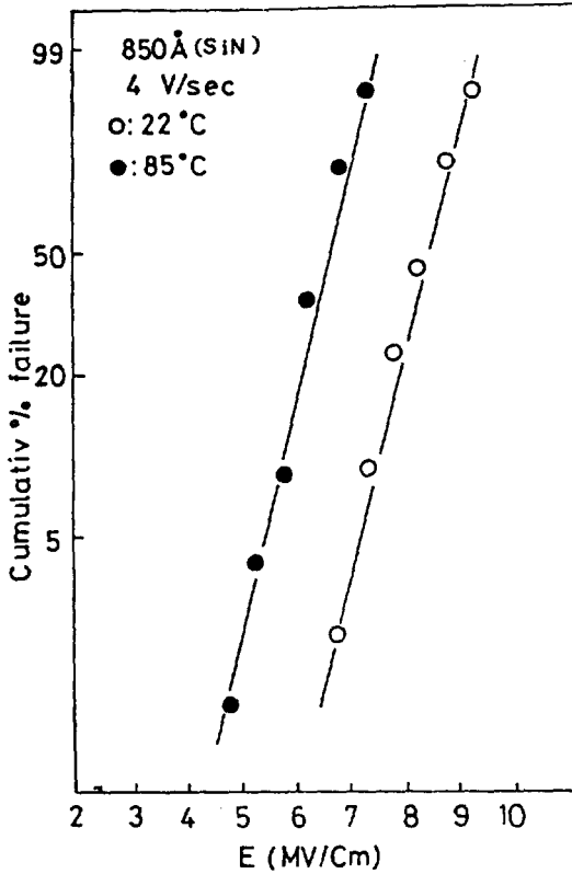
Fig. 5. Weibull distribution of breakdown strength.
