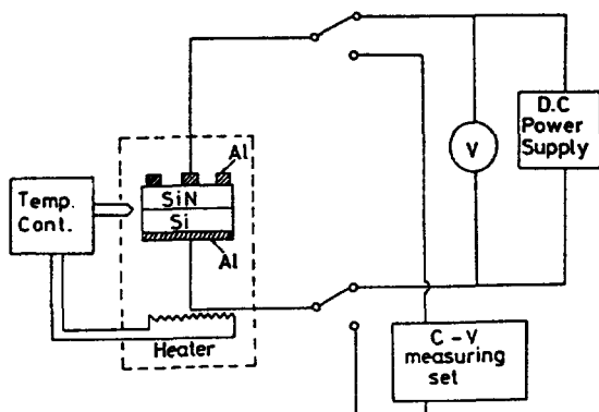
Fig. 2. Schematic diagram of D.C. stress and C-V measuring system.
